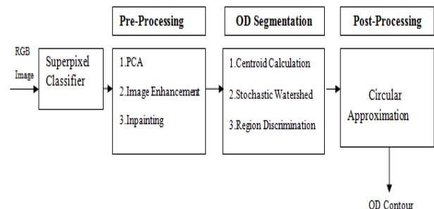
Figure 1: Block diagram optic disc segmentation
