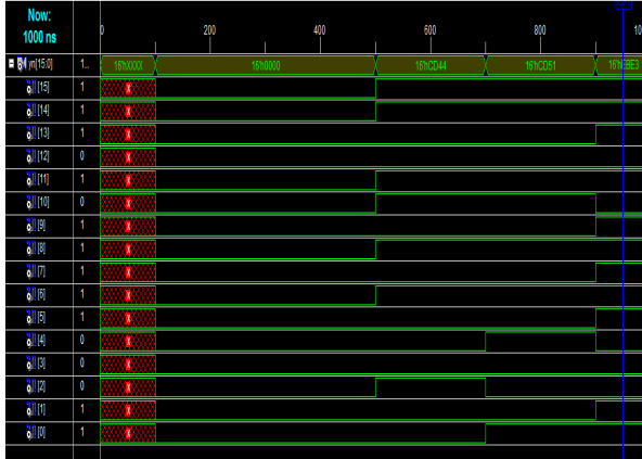
Figure 7: Output waveform of Pipelined FIR filter
