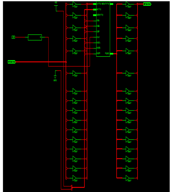
Figure 6: Schematic diagram of Pipelined FIR filter
