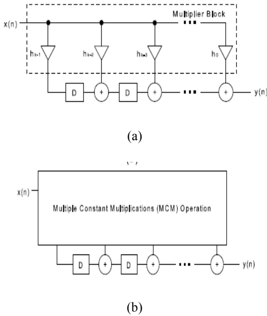
Figure 1: FIR filter implementations. (a) Transposed form. (b) Transposed form with an MCM block.
