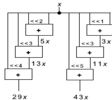
Figure 3: Shift-adds implementation of 29x and 43x (without partial product sharing)
