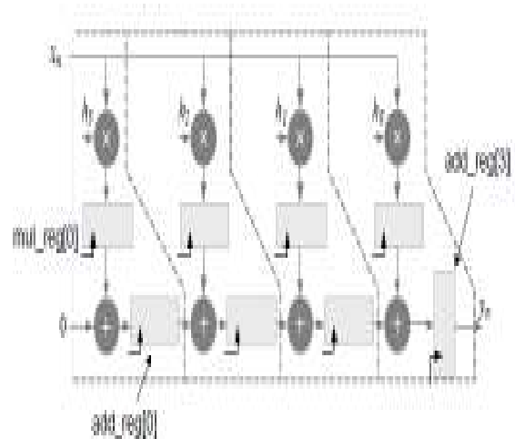
Figure 5: Pipelined FIR filter structure
