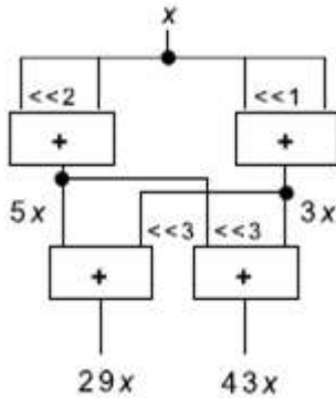
Figure 4: CSE algorithm (with partial product sharing)
